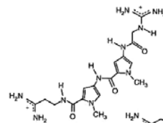
Netropsin
