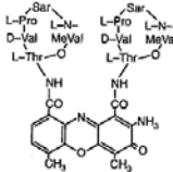
Actinomycin D
