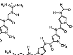
Distamycin A
